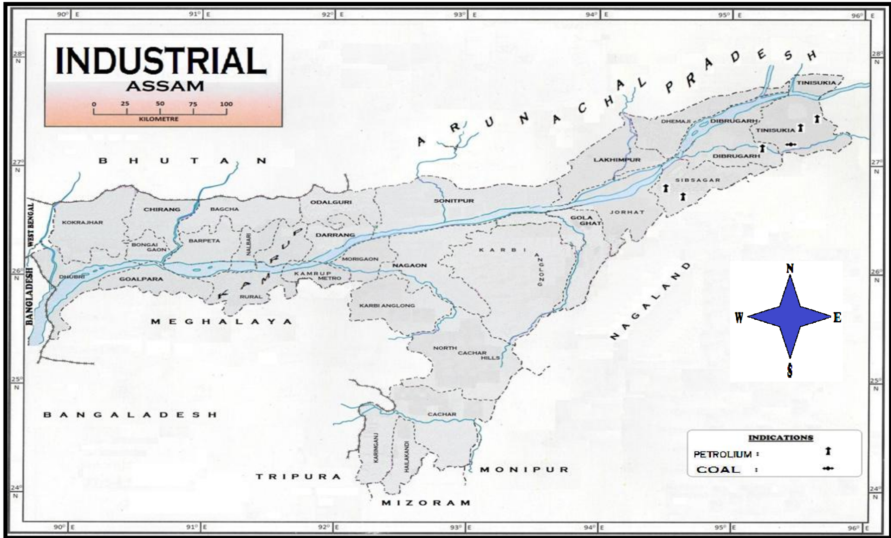
MAP – 3 : Location of Oil and Coal Mines in Assam
